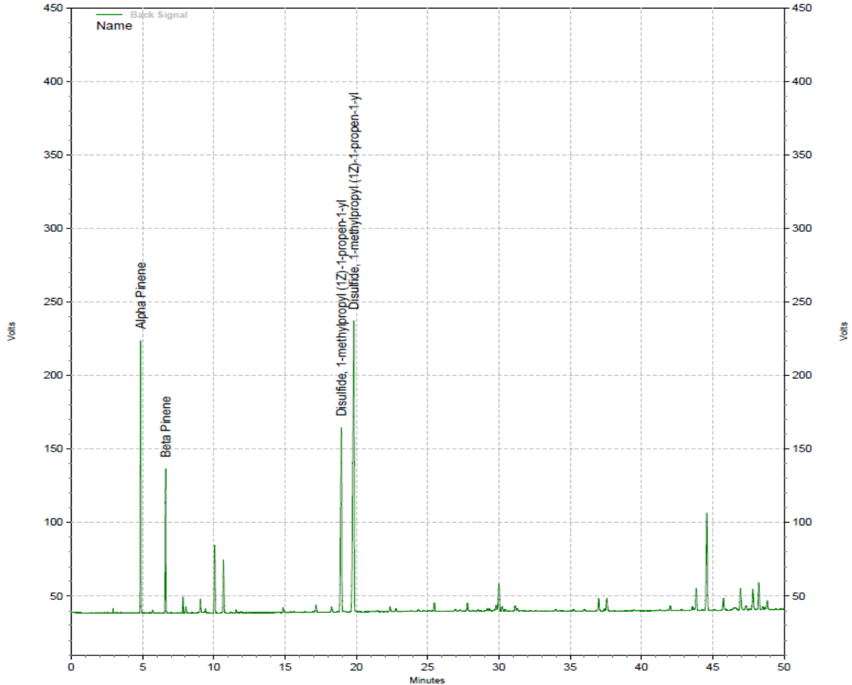
Representative Chromatogram of Asafoetida Oil (2342092803).
