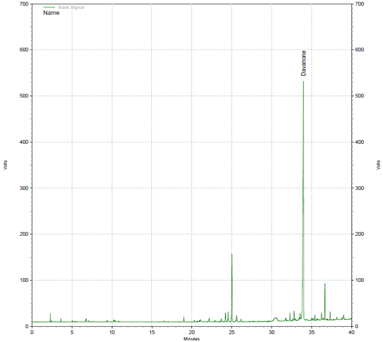
Representative Chromatogram of Davana Oil (2342122603).
